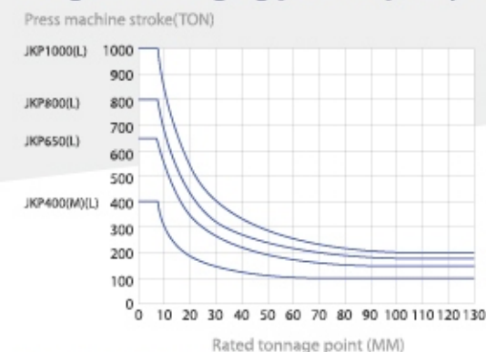
Diagram of forging press Capacity
