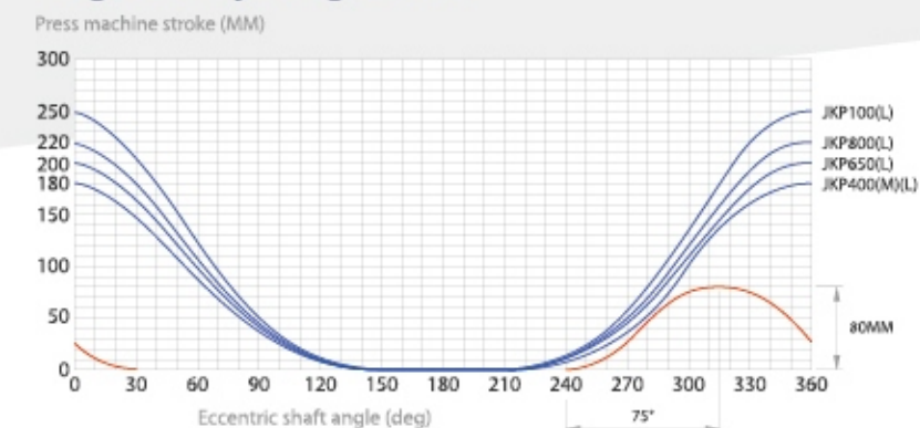
Diagram of ejecting stroke
